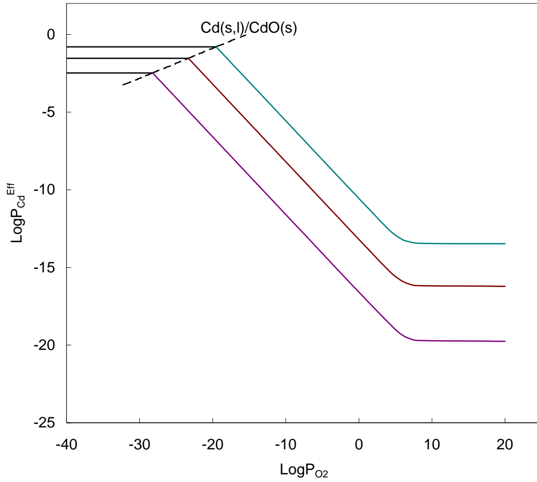
Total Cd-bearing Species Pressure, P_{\text{Cd}}^{\text{Eff}} , in the Cd-O System
