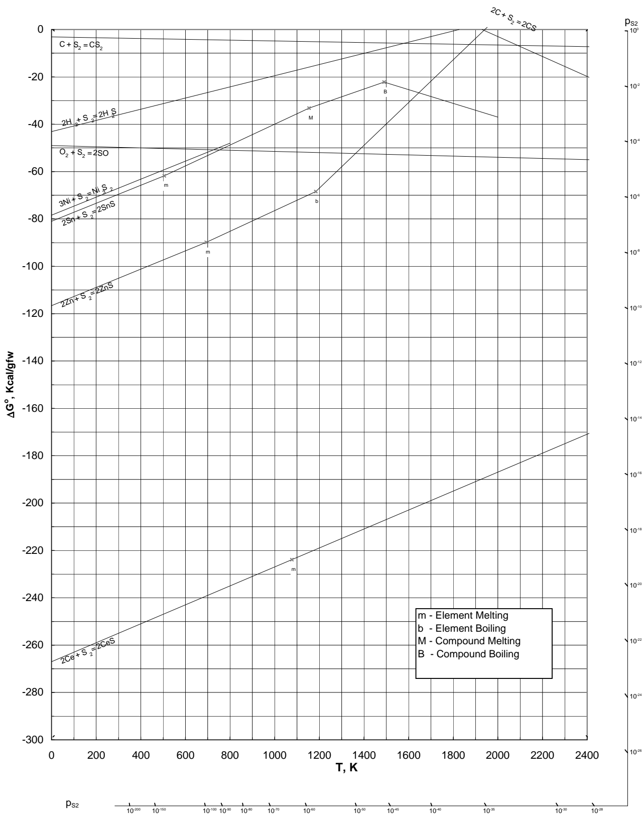
Ellingham Diagram for Selected Sulfides: Part-1
