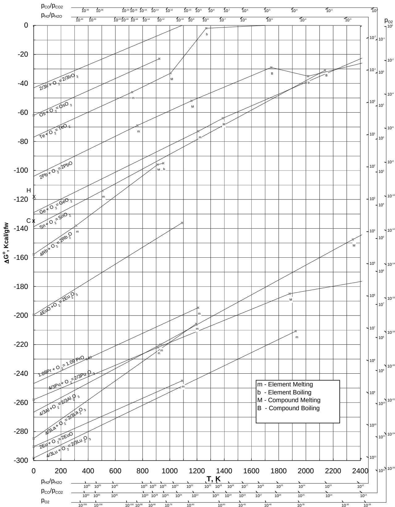
Ellingham Diagram for Selected Oxides: Part-5
