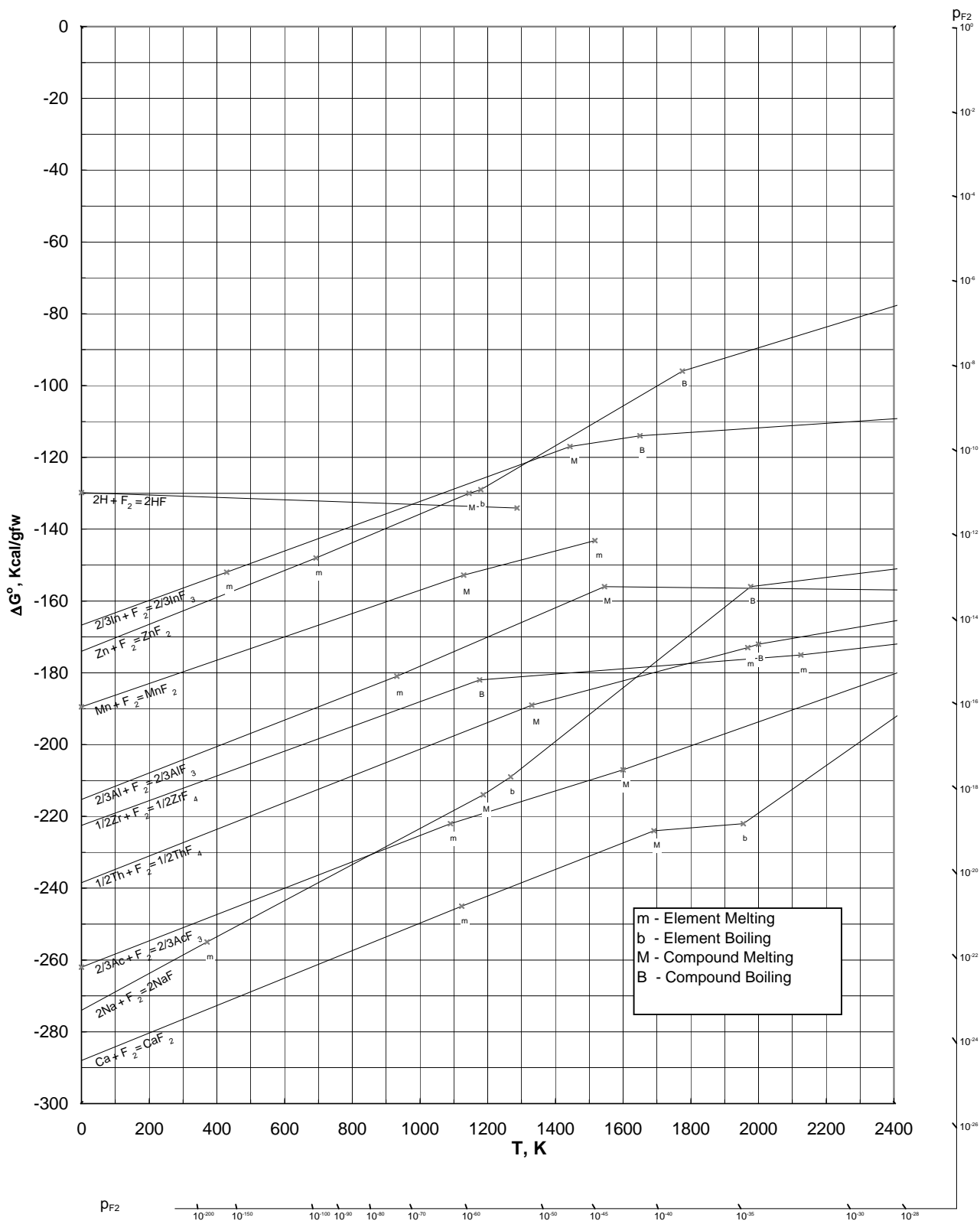
Ellingham Diagram for Selected Fluorides: Part-5
