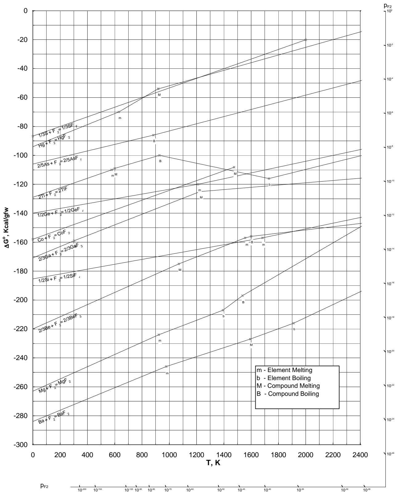
Ellingham Diagram for Selected Fluorides: Part-3
