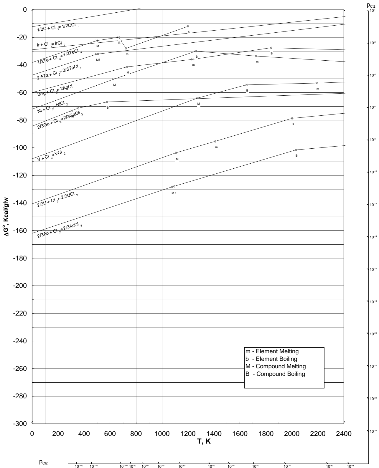
Ellingham Diagram for Selected Chlorides: Part-1
